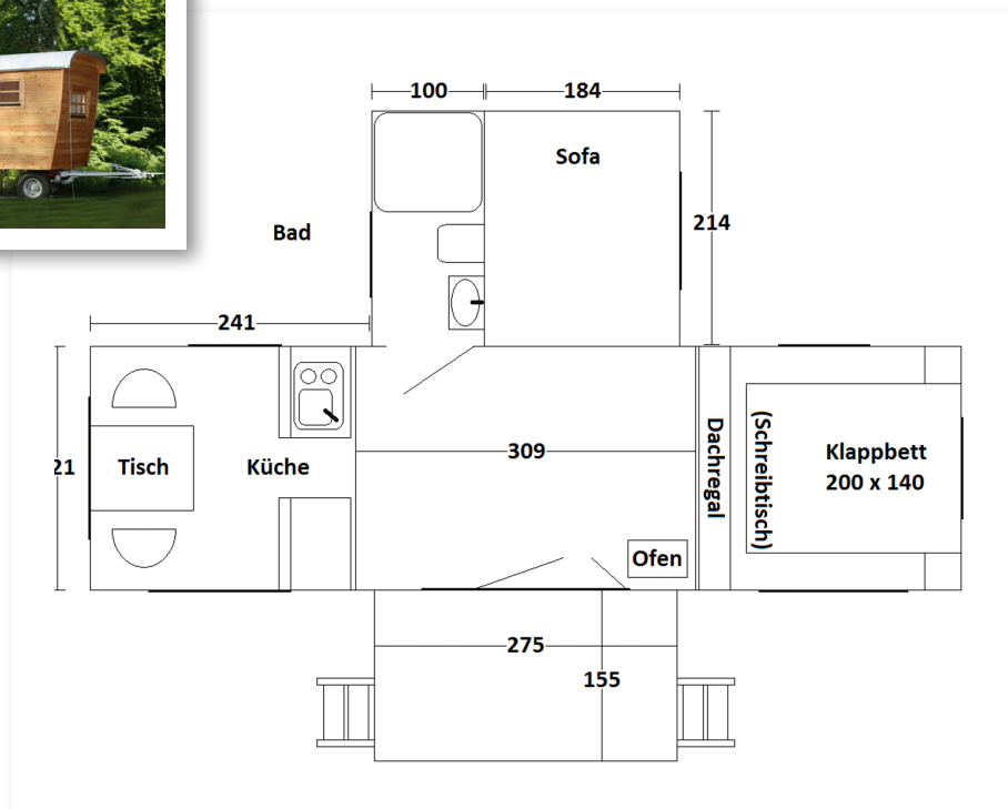
Grundriss Wohlwagen Basic. Innenmaße in cm.
